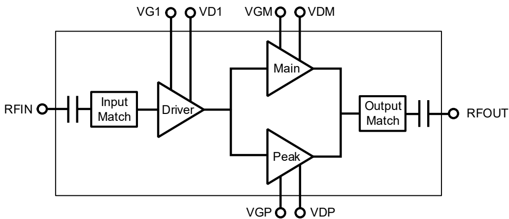
Figure 2. GNNM3542LN Block Diagram
