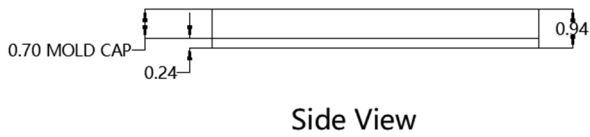
Figure 8. GNNM3542LN Package Dimension
