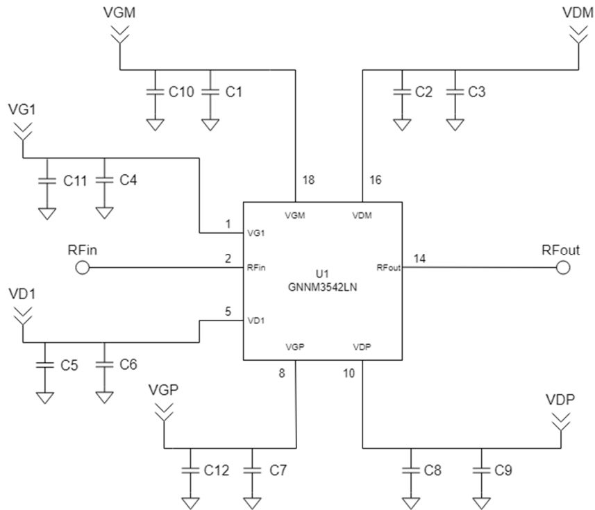
Figure 7. GNNM3542LN Application Schematic
