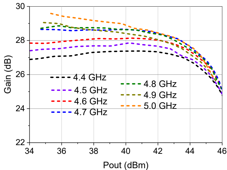
Figure 5. Measured Gain versus Output power (Pulse CW, 10us Pulse Width, 10% Duty Cycle)
