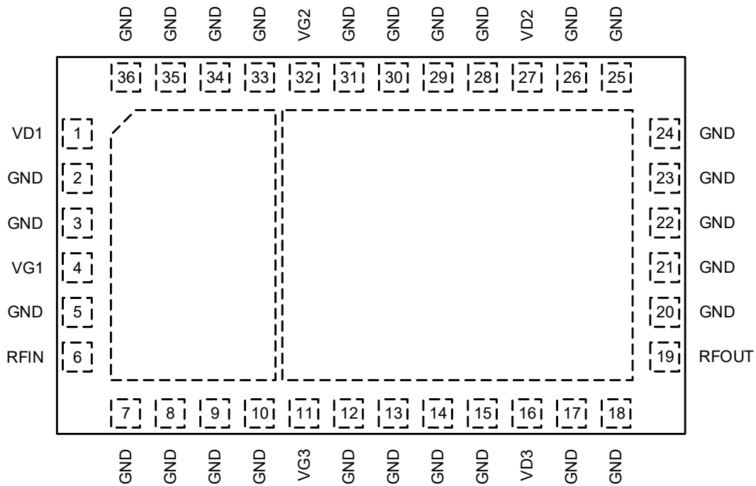
Figure 3. GNNM4945LA Pinout (Top View)
