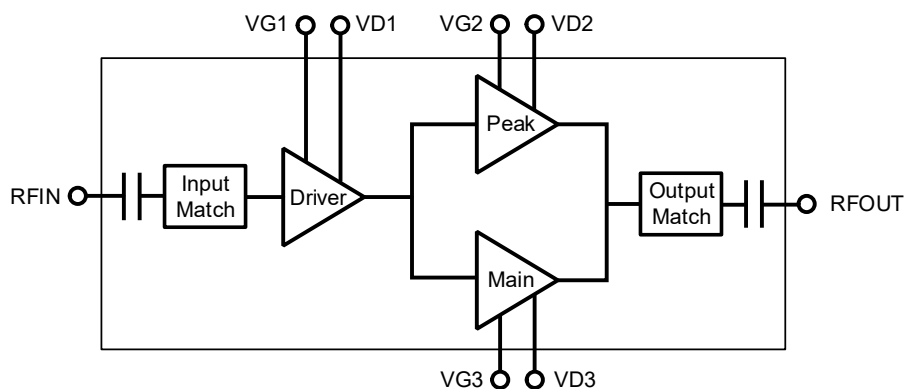
Figure 1. GNNM4945LA Block Diagram
