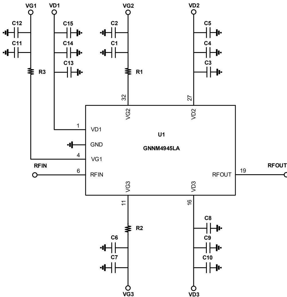
Figure 7. GNNM4945LA Application Schematic
