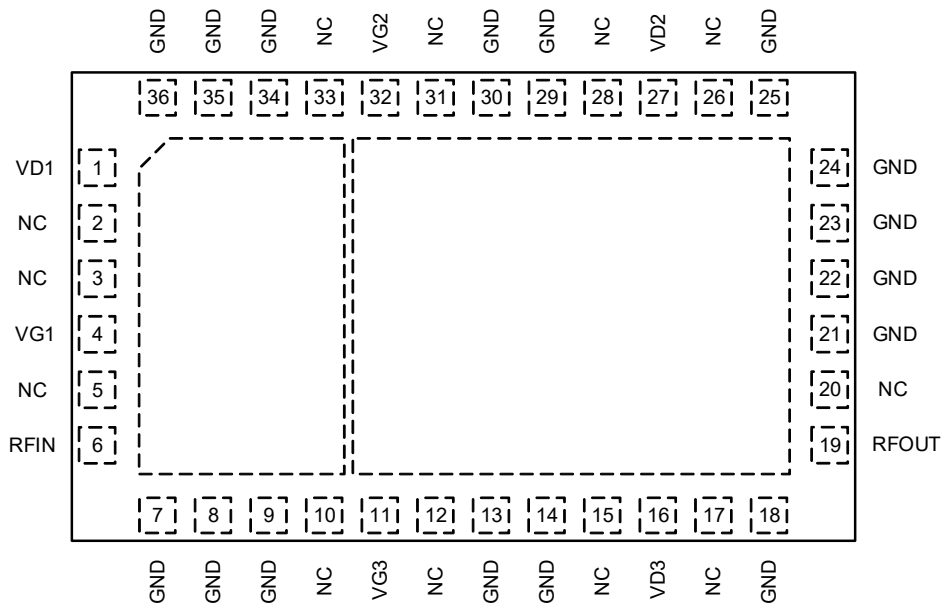
Figure 3. GNHM4949LE Pinout (Top View)
