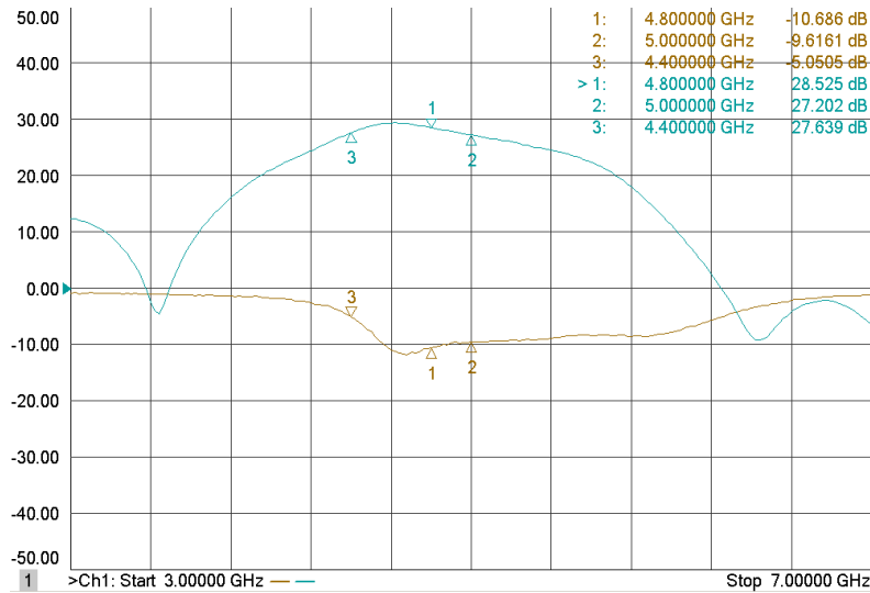
Figure 4. Measured S-parameters from 3 to 7 GHz
