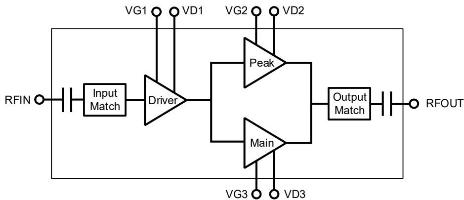
Figure 1. GNHM4949LE Block Diagram
