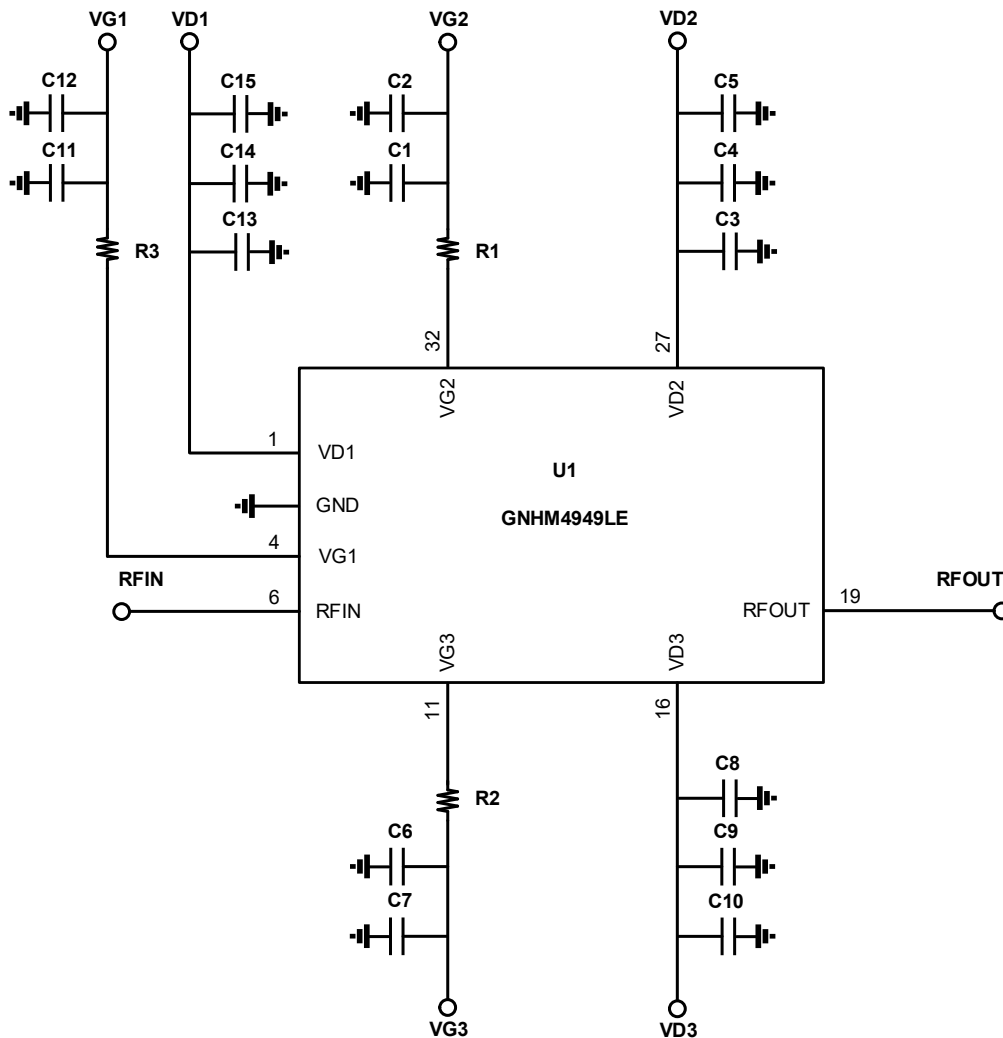
Figure 7. GNHM4949LE Application Schematic
